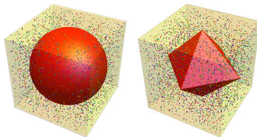
FIGURE 1. What is the probability to hit the ball? What is the probability to hit the octahedron?
