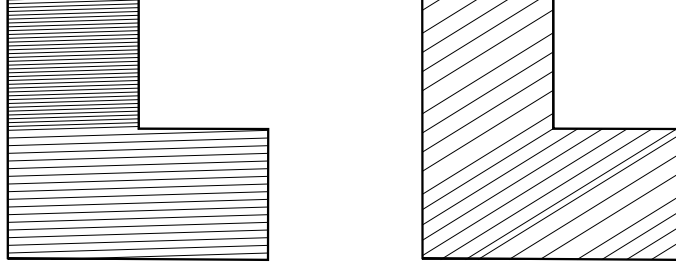
Figure 4. Periodic geodesics near slopes s = 0 and s = 1 .
