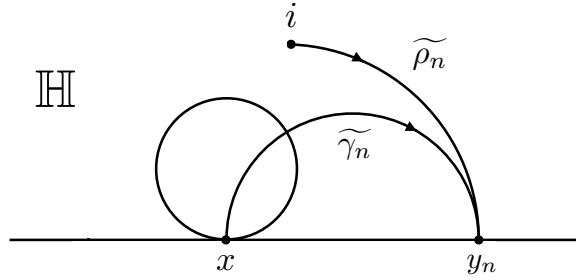
Figure 3. The geodesic \tilde{\rho}_n is close to \tilde{\gamma}_n outside a horoball neighborhood of the cusp x .
