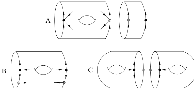
Figure 5. Results of splitting along a loop in the spine.
