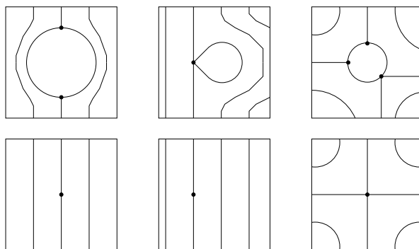
Figure 4. Contracting the boundary.
