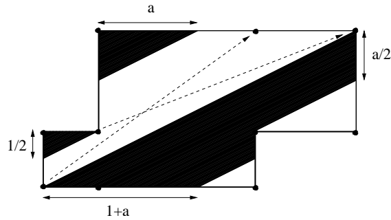
Figure 7. The foliation with slope 1/2 gives the connected sum of a pair of tori with irrational foliations.
