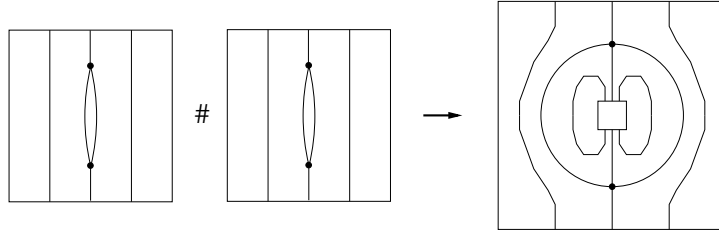
Figure 3. Local picture of the connected sum X_A \# Y_B .
