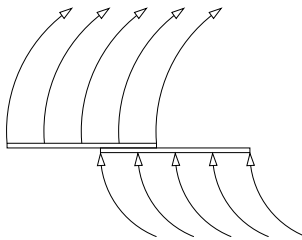
Figure 2. Leaves of \mathcal{F}_\rho and the first return map.
