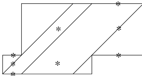
Figure 8. The spine of the foliation of slope 1 contains a pair of Weierstrass points.
