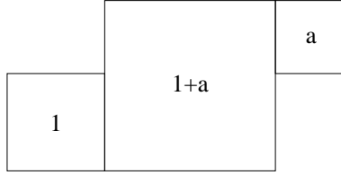
Figure 1. The polygon S(a) built from 3 squares.
