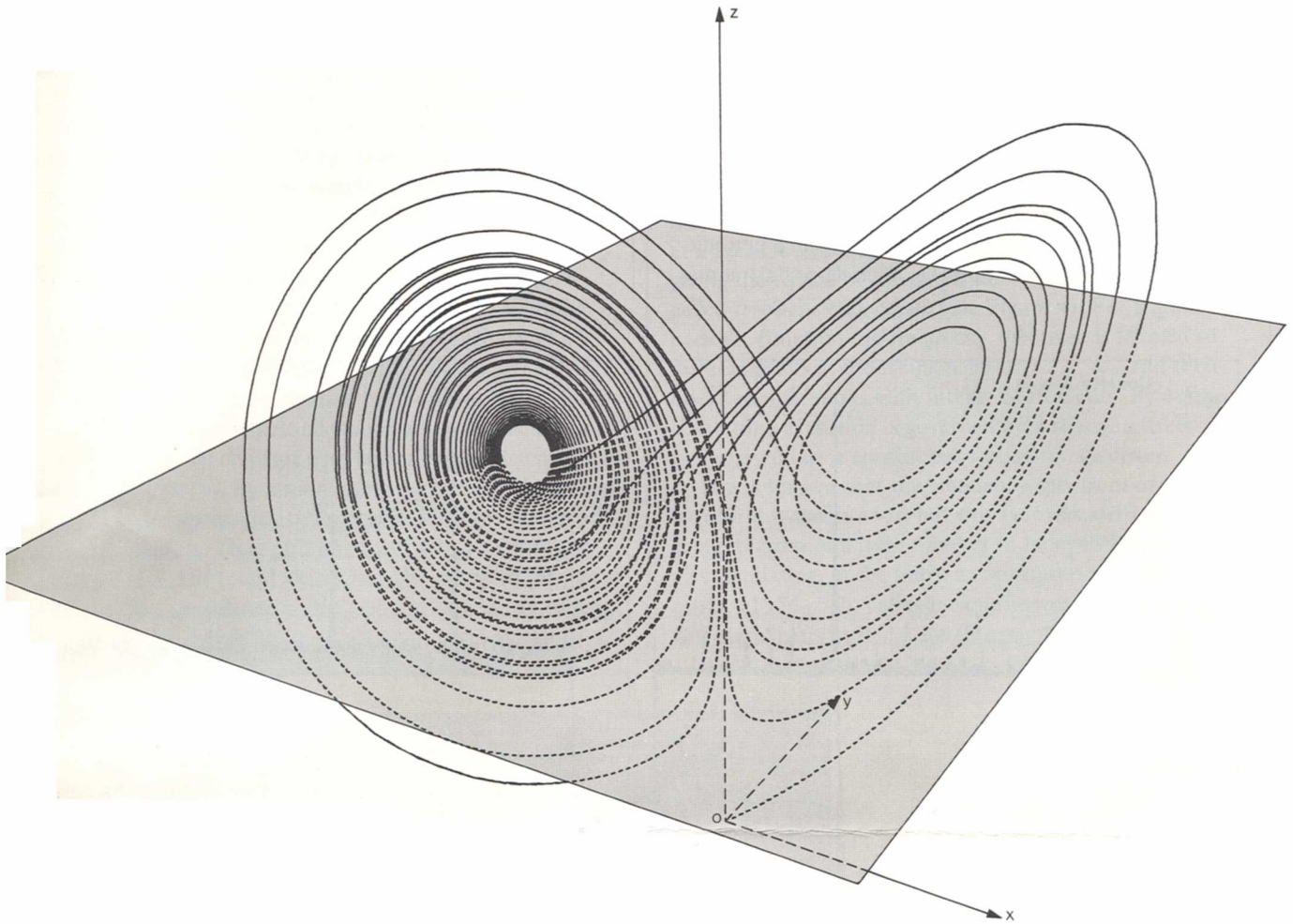
Figure 3. The Lorenz attractor. This beautiful figure has been obtained by Oscar Lanford, of Berkeley. It illustrates a new strange attractor, the Lorenz attractor , which is approached by the solutions of the Lorenz system of equations:
