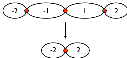
Figure 2. Topology of a cubic polynomial.
