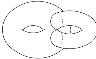
Figure 4. A connected sum resulting in a double zero.
