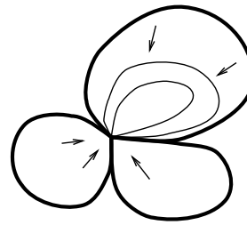
parabolic basin
