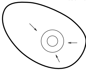
attractive basin
