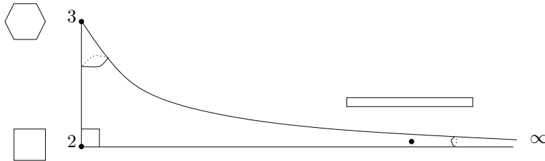
Figure 2. The moduli space of a torus, \mathcal{M}_1 = \mathbb{H}/SL_2(\mathbb{Z}) .
