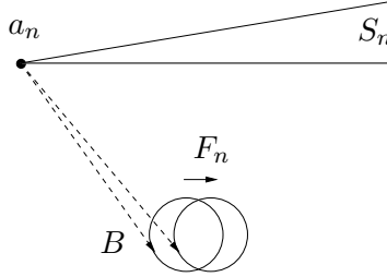
Figure 3. Horocyclic dynamics.
