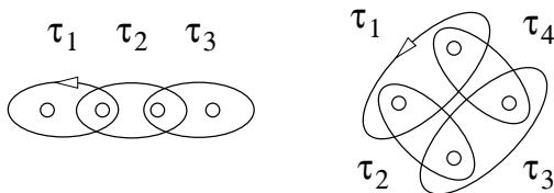
Figure 4. Right twists generating the braid group.
