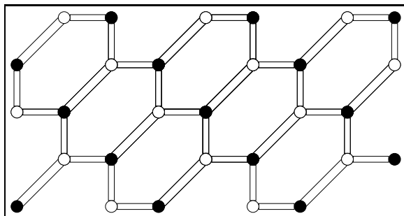
Figure 7. A model for the branched covering X .
