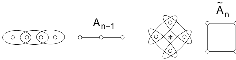
Figure 8. The braid groups of n points in \mathbb{C} and \mathbb{C}^* correspond to the Coxeter diagrams A_{n-1} and \tilde{A}_n .
