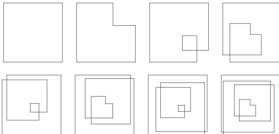
Figure 14. Immersed disks for 1 \leq g \leq 8 .
