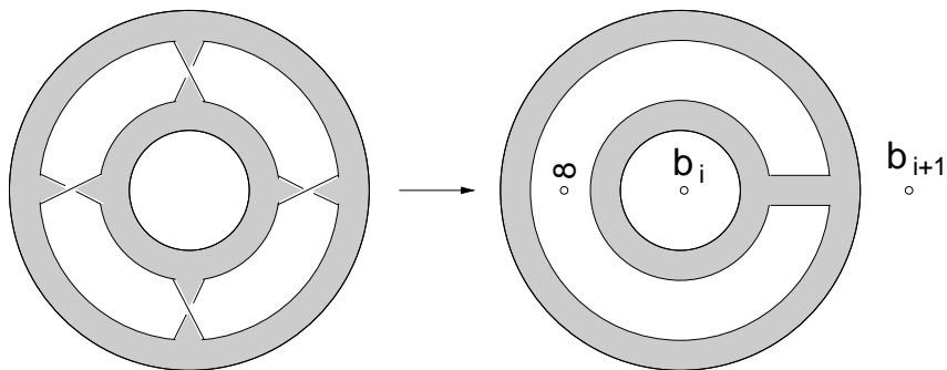
Figure 5. The surface X_i is built from the \mathbb{Z}/d -covering space of a pair of pants in \hat{\mathbb{C}} by capping off the inner and outer circles at the left with disks.
