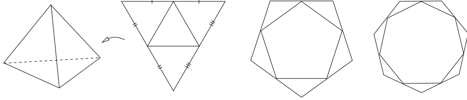
Figure 13. The sphere with the flat metric |dx|/|x^n - 1| , n = 3, 5, 7 .
